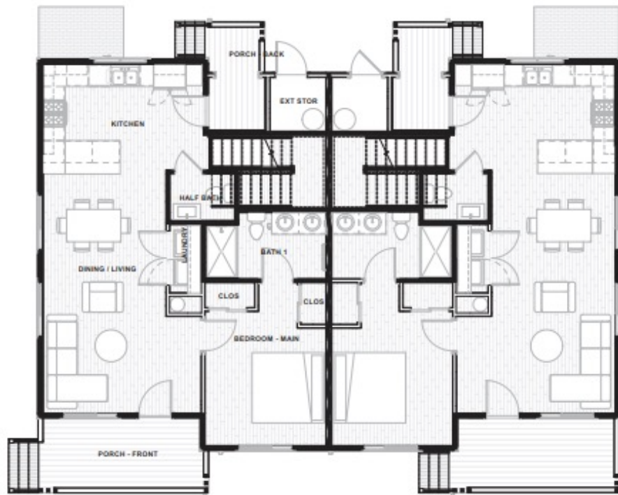
① First Floor - McDougald 1/4" = 1'-0"
