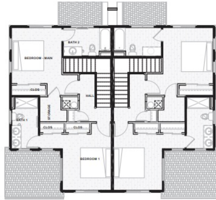
2 Second Floor - Pulley 1/8" = 1'-0"
